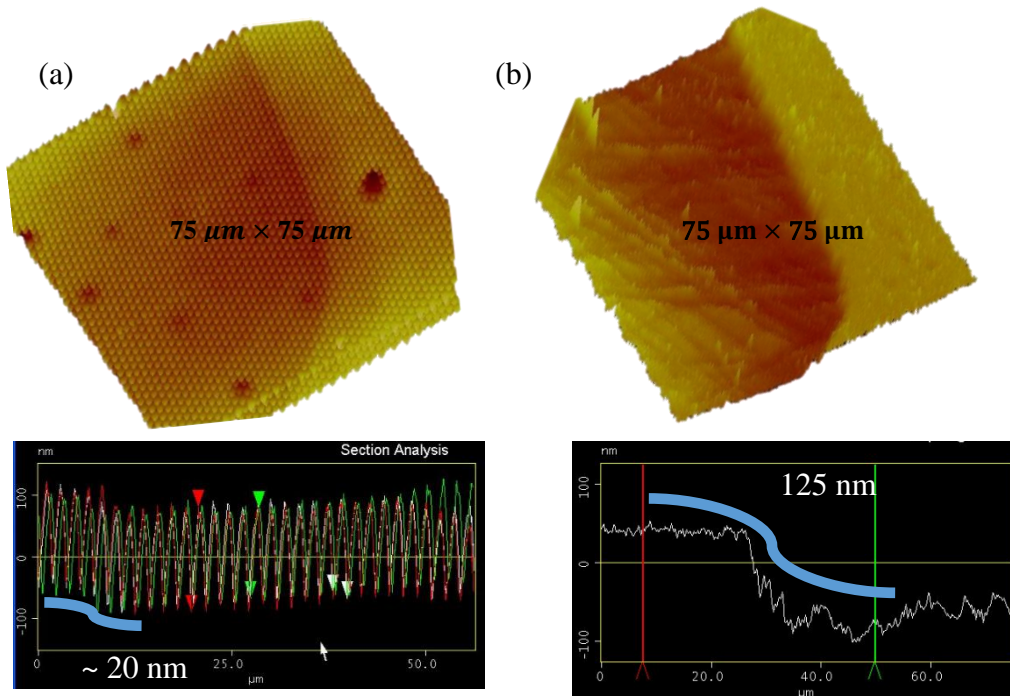
Figure 2.20: (a) Protruded Cu on NIM 58 with ~ 20 nm step and (b) Protruded Cu on NREL with ~ 125 nm step. Both scans are performed on (75 \mu\text{m} \times 75 \mu\text{m} ).
