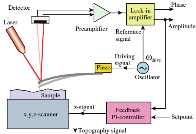
Figure 1.15: Schematic for the dynamic mode AFM [43]
