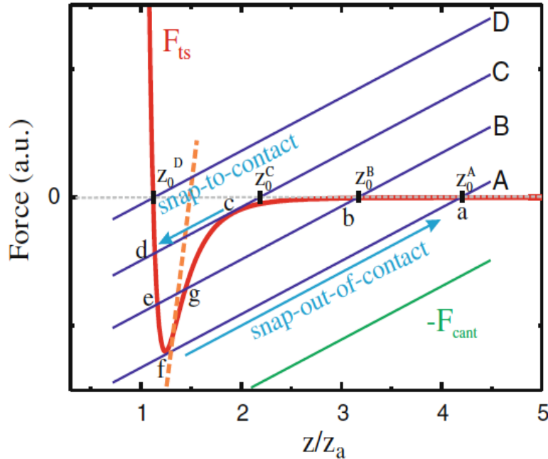
Figure 1.11: Force curve showing snap to/out of contact behavior of tip and sample surface [43]
