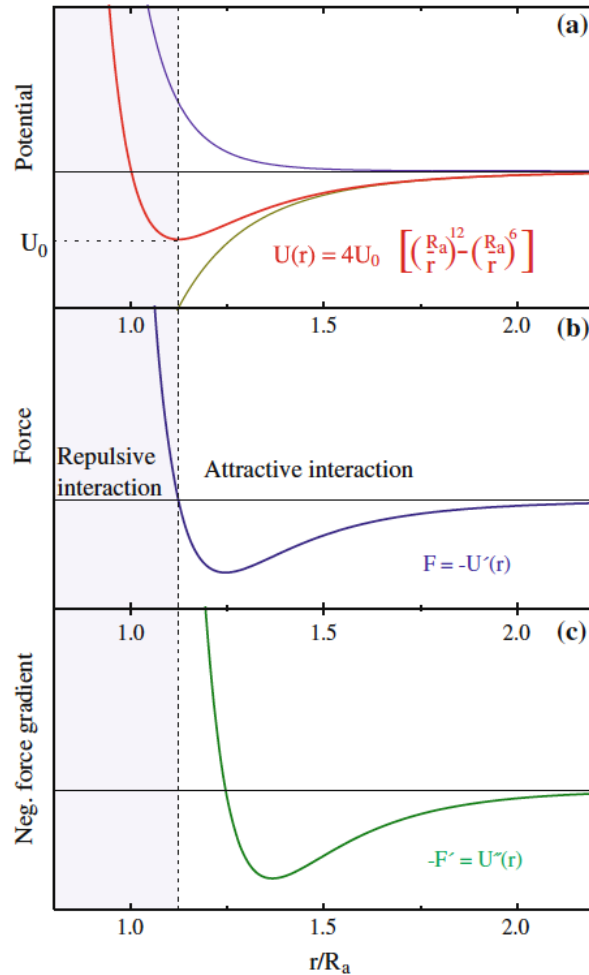
Figure 1.10: (a) Lennard Jones (L-J) Potential, (b) Force, (c) Force gradient plot for tip sample interaction [43]
