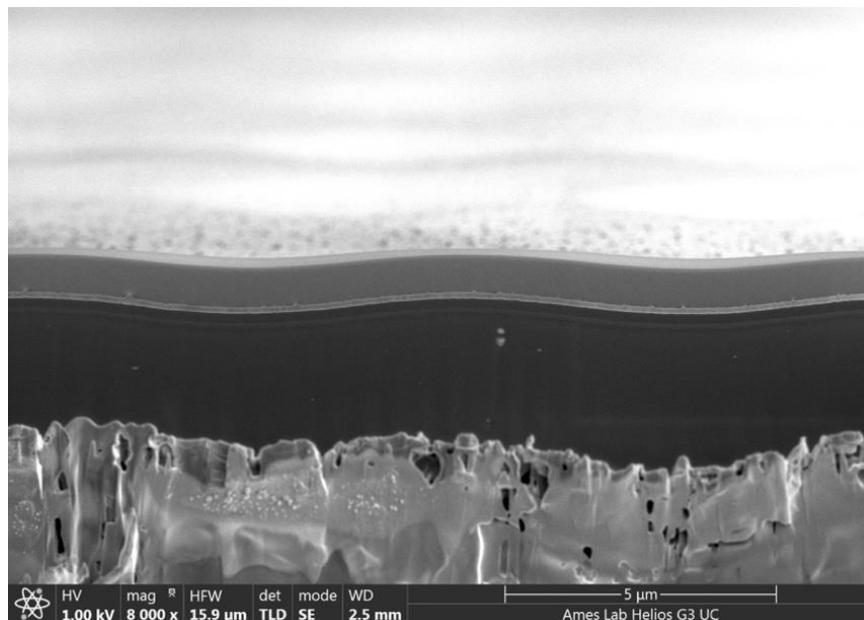
Figure 5.6: FIB image of the conformal WOLED on micro-patterned PET
