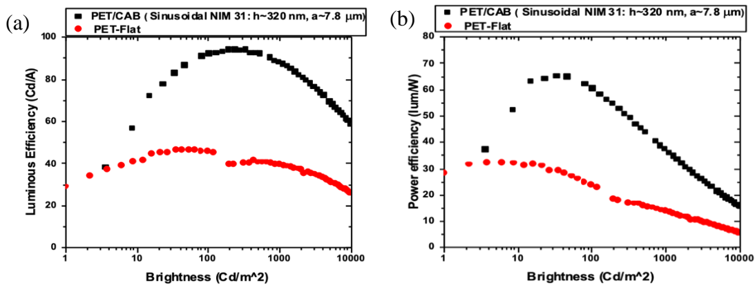
Figure 5.4: (a) \eta_L - L curve ; (b) \eta_P - L curve
