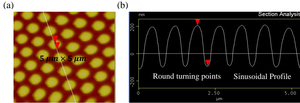
Figure 3.6: (a) NREL Patterned PC-MOBAY ( 5 \mu\text{m} \times 5 \mu\text{m} ) and (b) Pattern Profile, its attributes highlighted.
