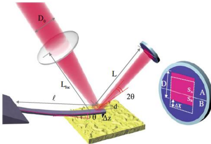
Figure 1.12: Beam deflection method used in AFM for cantilever bending[43]
