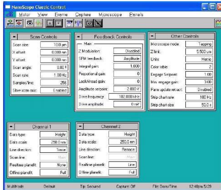
Figure 1.17: Nanoscope Interface for Tapping mode AFM [48]
