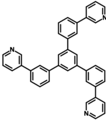
Figure 4.7: TmPyPB molecule [19]
