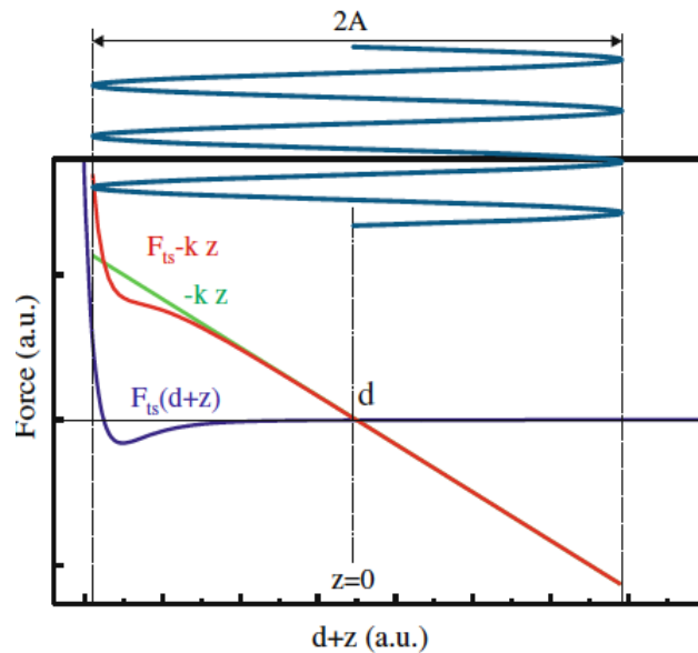
Figure 1.16: Force distance curve showing Intermittent/tapping mode characteristics [43]
