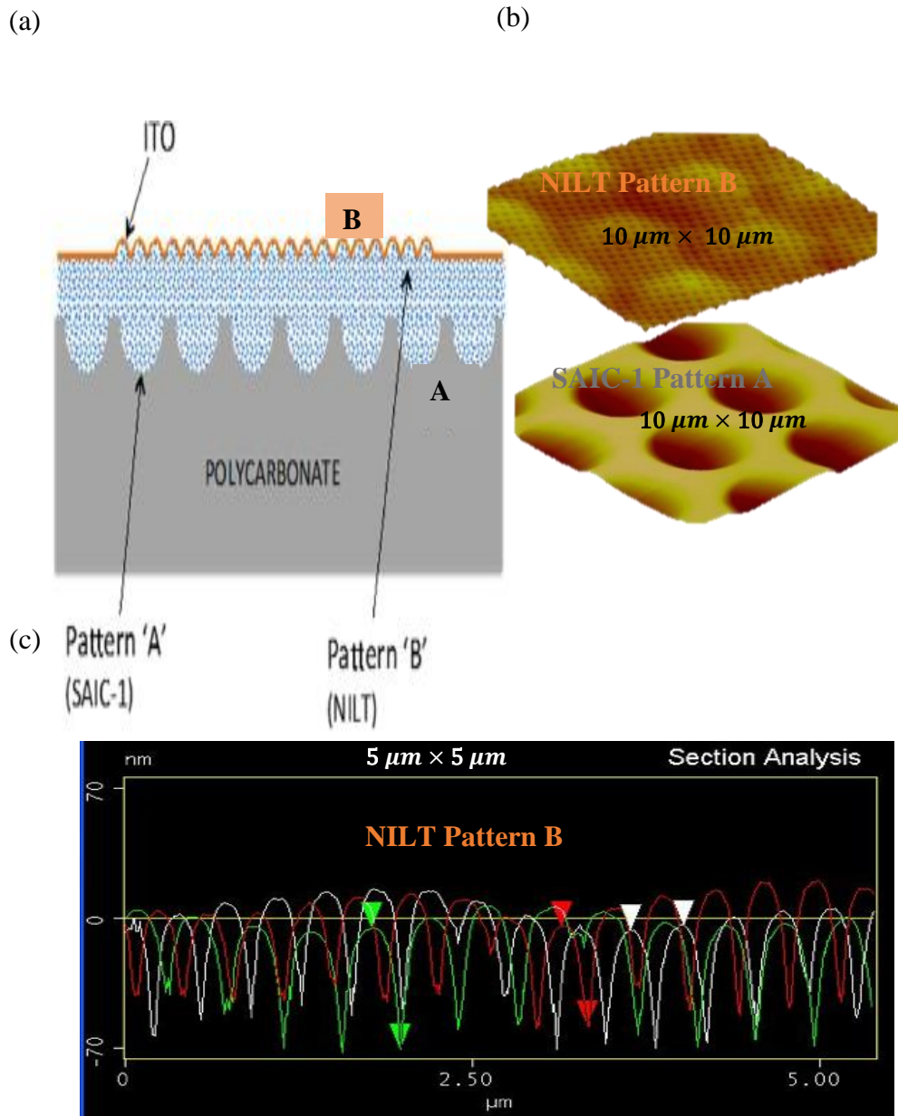
Figure 2.10: (a) Schematic for the dual corrugation, (b) AFM images for the NILT pattern (top) and SAIC-1 pattern (bottom) and (c) Section profile for NILT pattern ( h \sim 50 \text{ nm} ; a \sim 380 \text{ nm} ).
