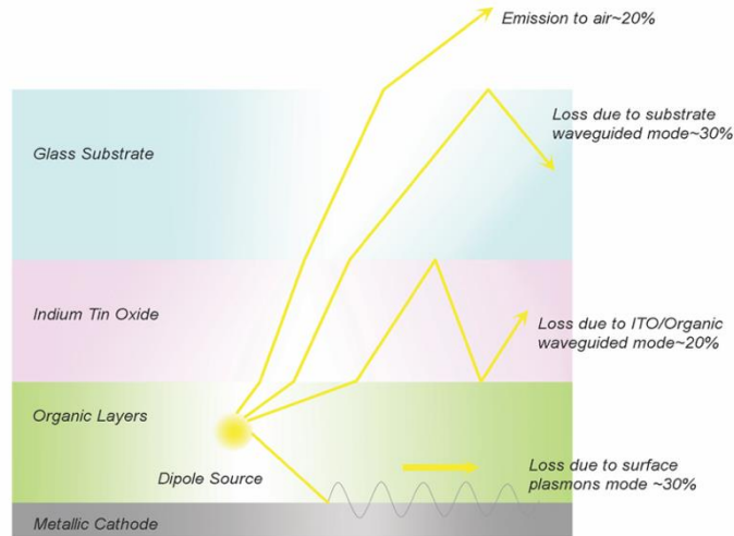
Figure 1.9: Schematic showing loss channels in OLED [35]
