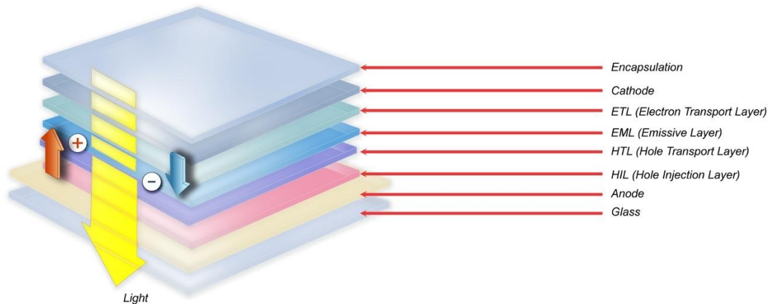
Figure 1.1: Schematic of an OLED with its various components
